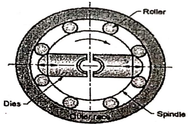
(b) Rotary swaging machine operation
